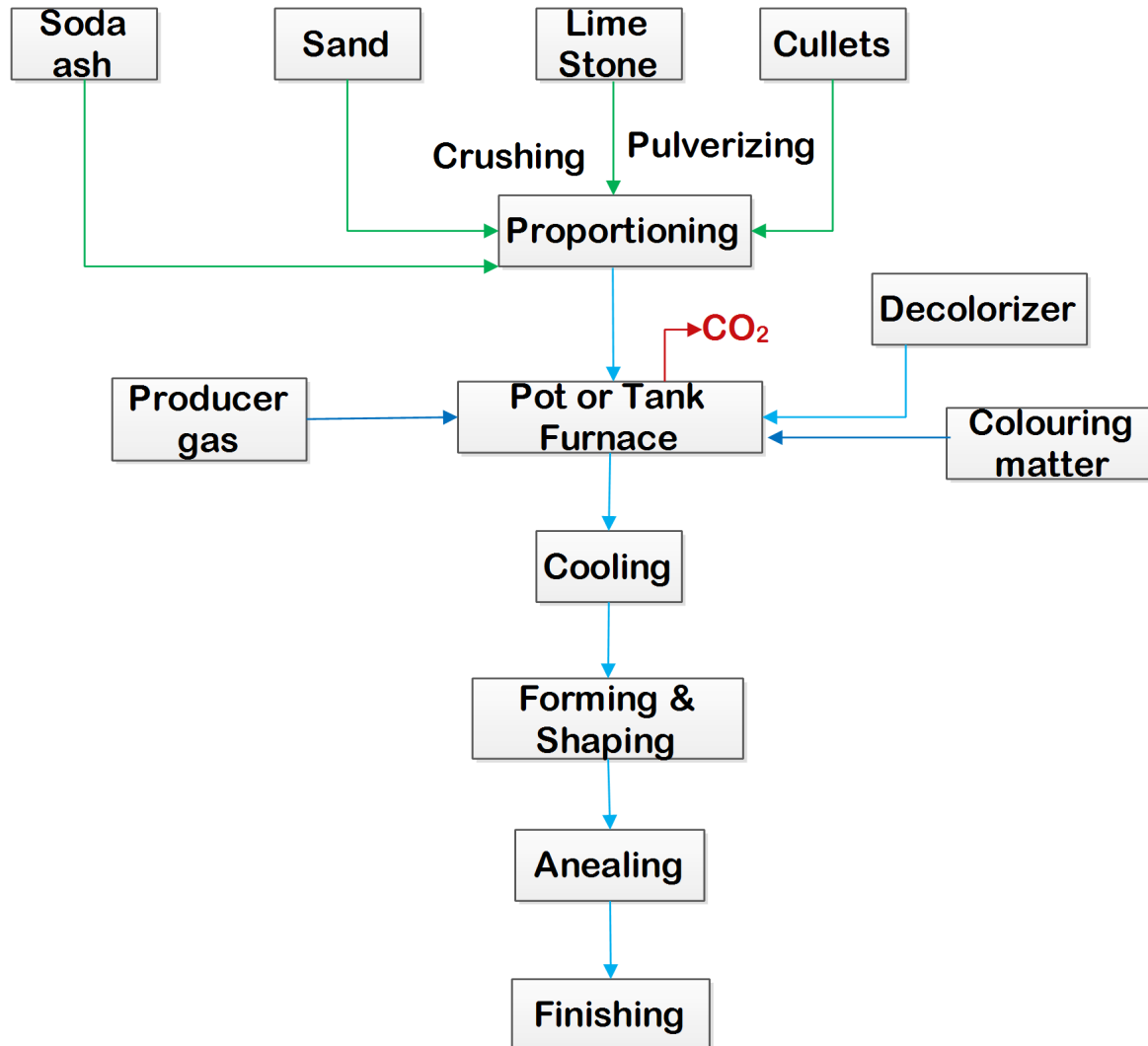
Figure: Manufacturing of Glass
